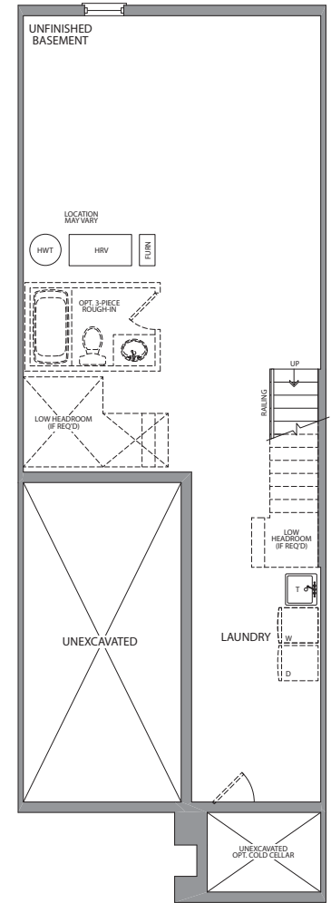
BASEMENT ELEVATION A & B
