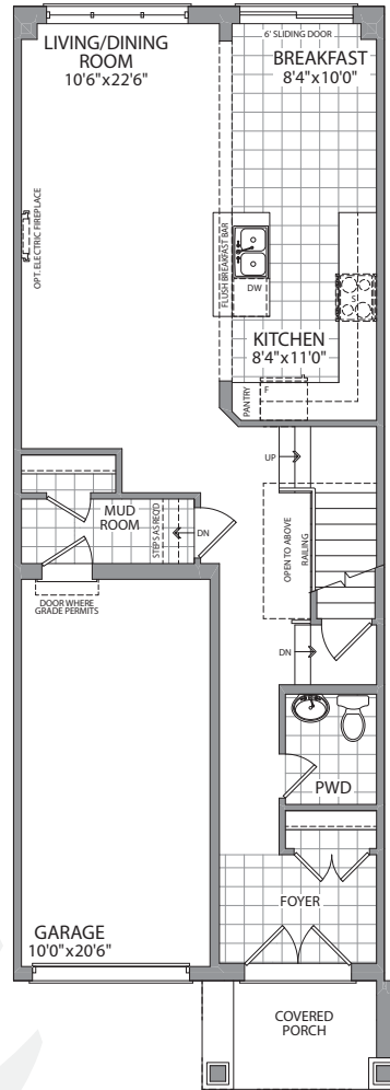
FIRST FLOOR ELEVATION A
