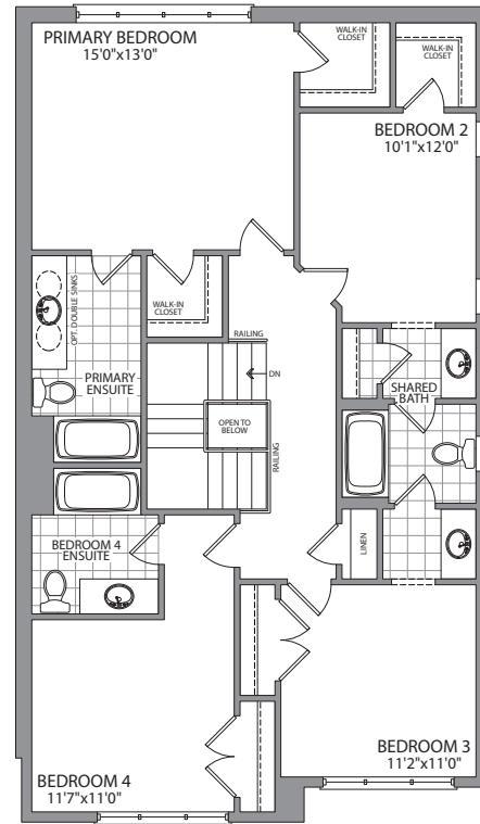
SECOND FLOOR ELEVATION A
