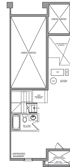
BASEMENT ELEVATION B2
