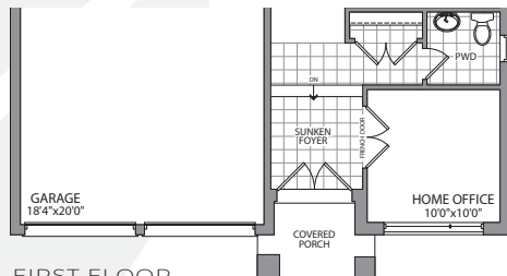
FIRST FLOOR ELEVATION C
