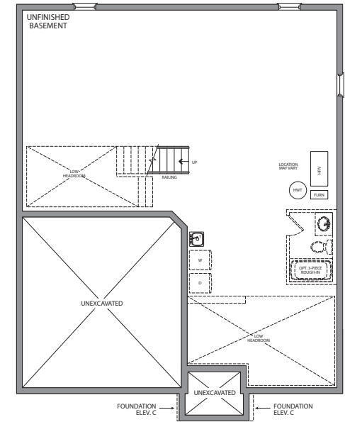
BASEMENT ELEVATION A, B & C
