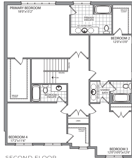
SECOND FLOOR ELEVATION A
