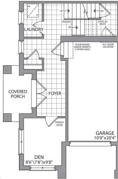
FIRST FLOOR ELEVATION A
