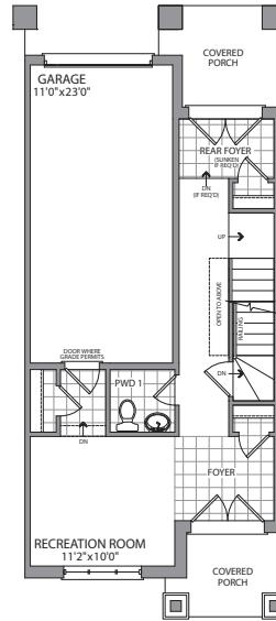
FIRST FLOOR ELEVATION A1-END
