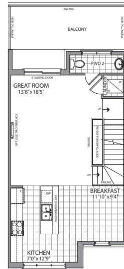
SECOND FLOOR ELEVATION B1-END
