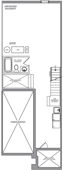
BASEMENT ELEVATION A & B1
