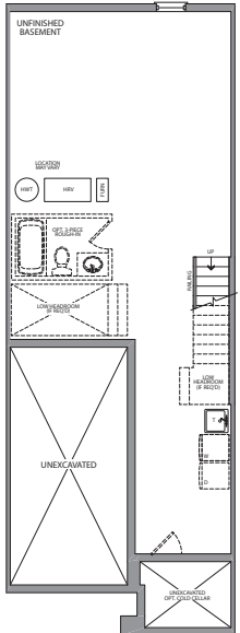
BASEMENT ELEVATION B2
