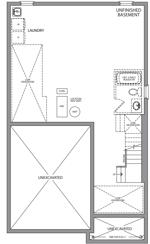
BASEMENT ELEVATION A & C
