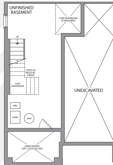
BASEMENT ELEVATION A & B
