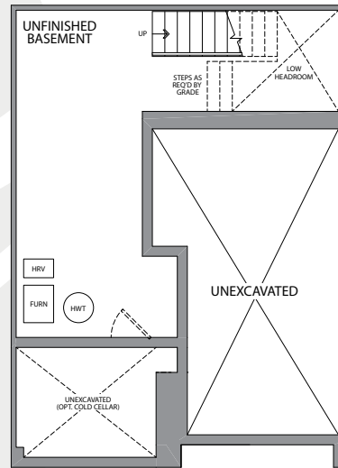
BASEMENT ELEVATION A & B
