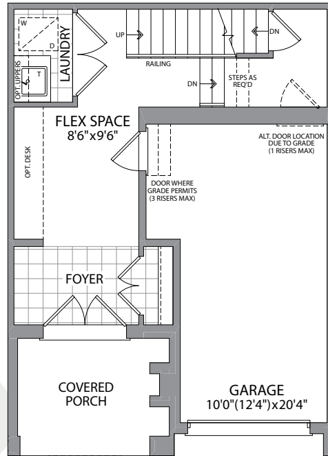
FIRST FLOOR ELEVATION A & B
